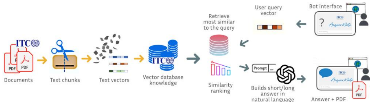
Figure 13: RAG-based process flow diagram for AnswerMate, developed by ITCILO
