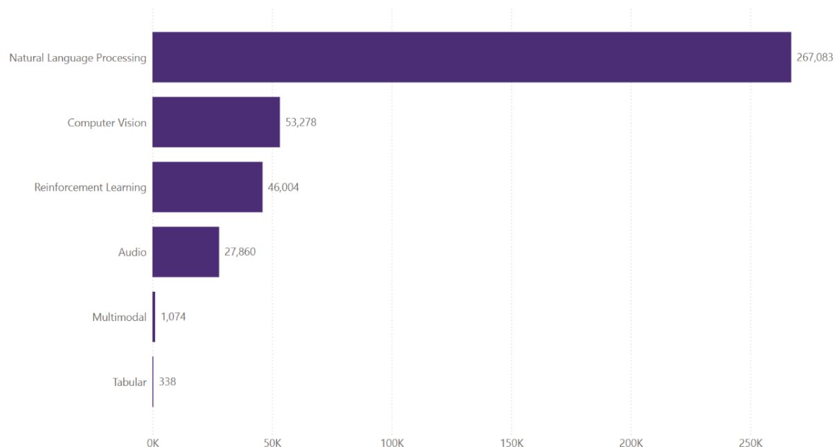
Figure 9: Statistics from models on Hugging Face by type of task
